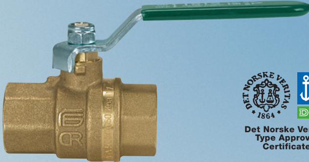
Art. 2411 1/4" "CR" alloy with steel lever from 1/4" to 4"
