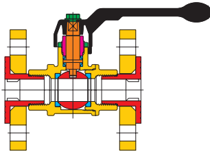
Art. 1216 with mobile flanges with lever in aluminium. Available range: from DN 15 to DN80
