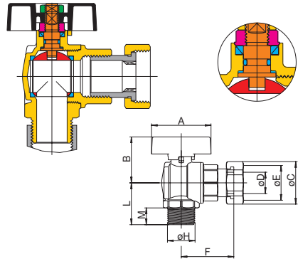
Art.2166R424 angle, male 1/2" ISO 228 / turnable nut 3/4" Art. 2168R405 angle, male 3/4" ISO 228 / turnable nut 3/4"
