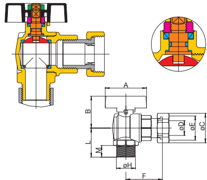
Art.2168G424 angle, male 1/2" ISO 228 / turnable nut 3/4" Art. 2168G405 angle, male 3/4" ISO 228 / turnable nut 3/4"
