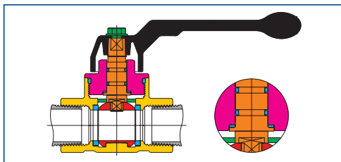
Art. 2330 F/F with extractable kit with lever in aluminium. Available range: 1/2" to 3/4"
