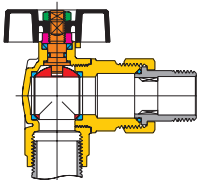
Art. 2077 F/Nut+tail with T-handle. Available range: from 1/2" to 1"
