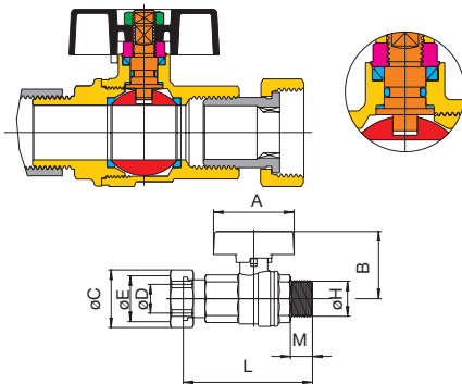
Art. 2162G424 male 1/2" ISO 228 / turnable nut 3/4" Art. 2164G405 male 3/4" ISO 228 / turnable nut 3/4"
