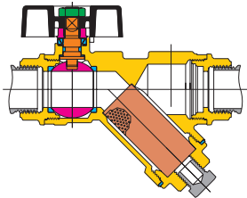
Art. 2435 F/F ISO 7/1 Rc "CR" alloy with handle from 1/2" to 1"
