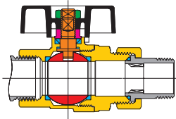
Art. 2037 F/Nut+tail with T-handle. Available range: from 1/2" to 2"
