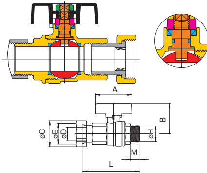
Art. 2162R424 male 1/2" ISO 228 / turnable nut 3/4" Art. 2164R405 male 3/4" ISO 228 / turnable nut 3/4"
