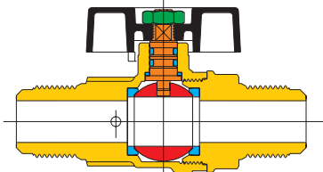
Art 4095 Flare/Flare SAE 45° with sealed side top. Available range from 3/8" to 5/8"
