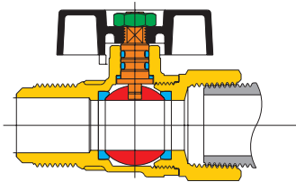
Art. 4092 - Art. 4093 Female NPT/SAE 45° copper end
