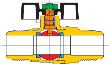
Art. 4091 Flare/Flare SAE 45°. Available range from 3/8" to 5/8"
