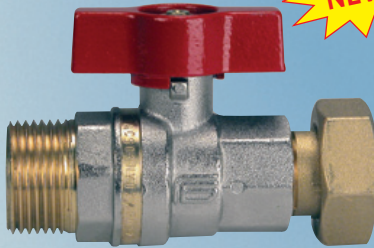
Art. 2162R424 male 1/2" ISO 228 / turnable nut 3/4" Art. 2164R405 male 3/4" ISO 228 / turnable nut 3/4"
