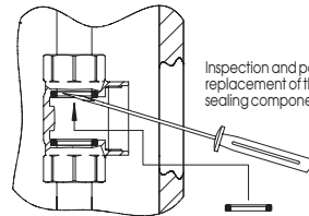
Ball extraction with valve open
