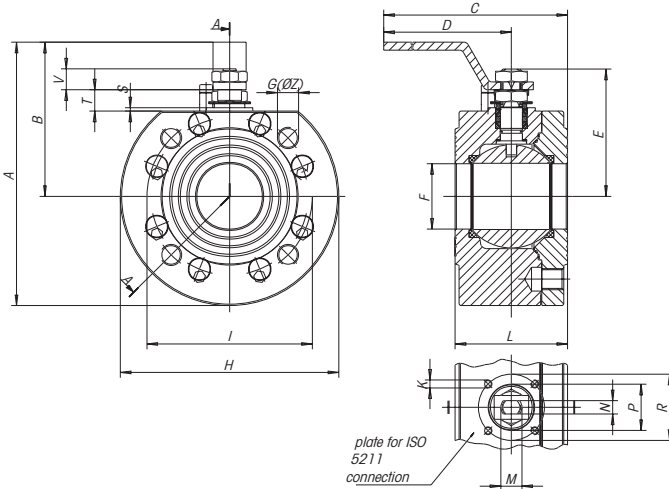
FLANGE DRILLINGS UNI2223-67
