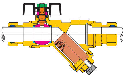
Art. 2435 Copper-Copper ends "CR" alloy with h-handle from 15 - 22 - 28 mm.
