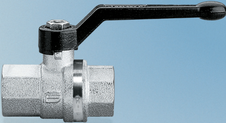
Art. 0501 F/F with lever in aluminium. Available range: from 1/4" to 4" Art. 0502 M/F with lever in aluminium. Available range: from 1/4" to 2" 1/2" Art. 0503 M/M with lever in aluminium. Available range: from 3/8" to 2"
