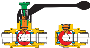
Art. 1100 3-way L-ported with lever in aluminium. Available range: from 1/4" to 2" Art. 1120 3-way L-ported with lever in aluminium. Available range: from 1/4" to 2"
