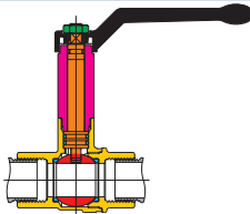
Art. 2170 F/F with lever in aluminium. Available range: from 1/2" to 2" Art. 2185 Available range 3/4" and 1"
