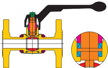
Art. 1206 3-piece bolted and flanged with lever in aluminium. Available range: from DN 20 to DN 100
