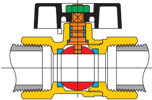
Art. 4097 F/F NPT Available range from 3/8" to 3/4"
