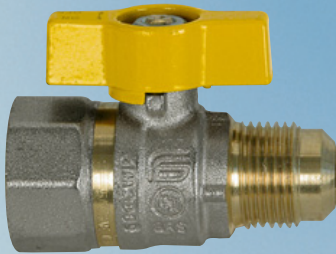
Art. 4092 - Art. 4093 Female NPT/SAE 45° copper end
