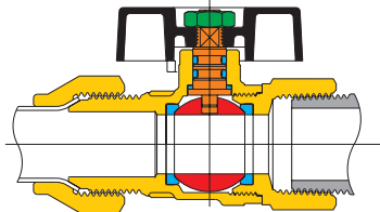
Art. 4949 (brass) Female ISO 7/1 Rp / Gas 60° copper end Art. 4950 (DZR) Female ISO 7/1 Rp / Gas 60° copper end
