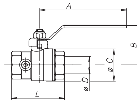
Art. 2375 F/F with turnable drain and aluminium lever from 1/2" to 2"
