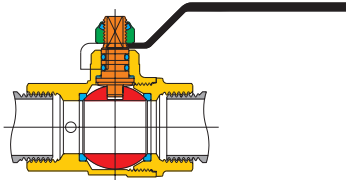
Art. 2374 F/F with drain and aluminium lever from 1/2" to 2"
