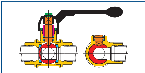
Art. 1150 3-way L-port with lever in aluminium. Available range: from 1/4" to 2"
