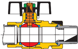
Art. 2047 F/Nut+tail with T-handle. Available range: from 1/2" to 1"
